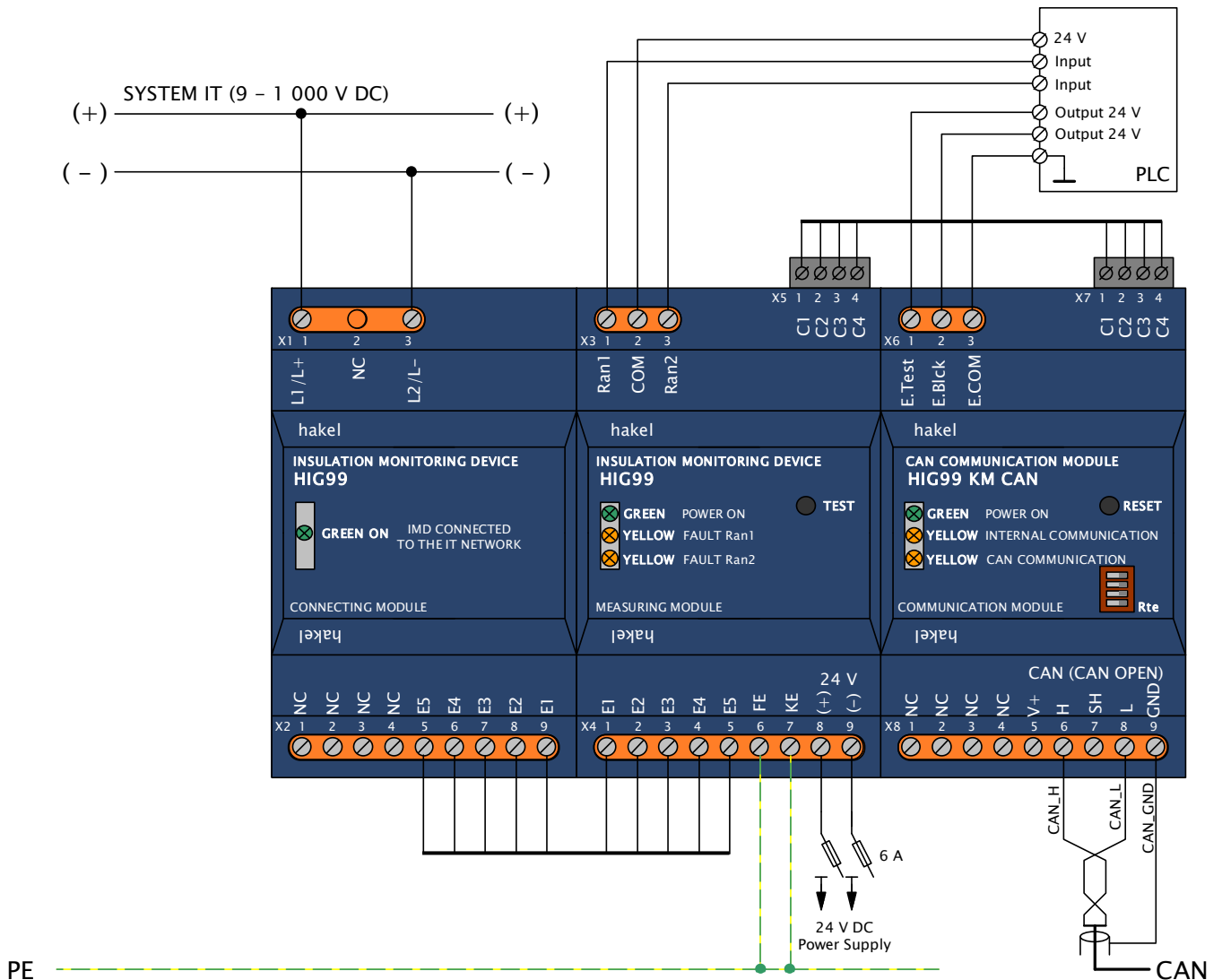
Picture 5. Direct IT power supply system's connection diagram
